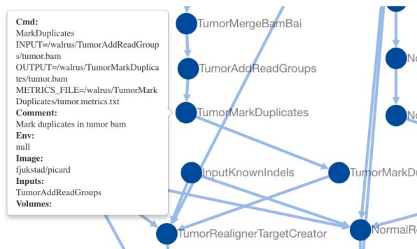
Figure 1. Screenshot of the web-based visualization in walrus. The user has zoomed in to inspect the pipeline step which marks duplicate reads in the tumor sequence data.
